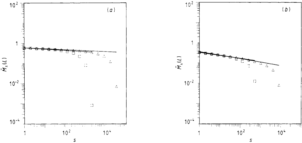
Figure 3. Plot of the quantity \tilde{M}_s(L) = \sum_{s'=s}^{\infty} \tilde{n}_{s'}(L) against s for different values of the lattice size L . Values for the cluster size exponent \tau obtained by fitting a straight line and using (3.9) are listed in table 1. ((a), (b) as in figure 2.)
