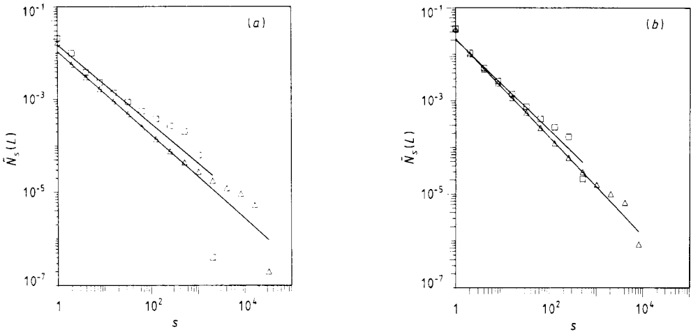
Figure 2. Plot of the quantity \tilde{N}_s(L) = \sum_{s'=s}^{2s-1} \tilde{n}_{s'}(L) against s for different values of the lattice size L . (a) Square lattice, L = 100 ( \square ), 500 ( \triangle ); (b) cubic lattice, L = 20 ( \square ), 60 ( \triangle ). Observe that the curves rise above the extrapolated straight line before falling off at large s due to the finite lattice size. Values for the cluster size exponent \tau obtained by fitting a straight line and using (3.7) are listed in table 1.
